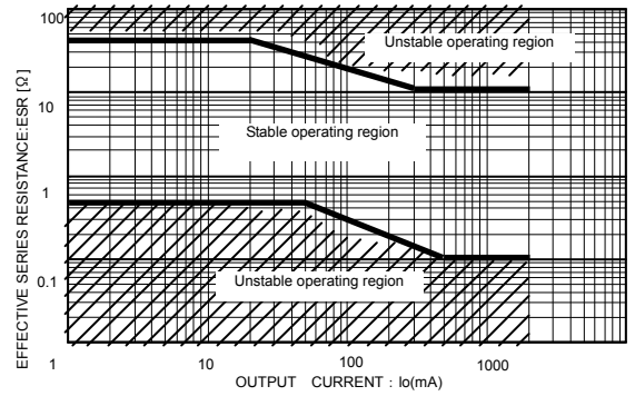
Fig.34 ESR vs Io Characteristics (BA□□DD0)
